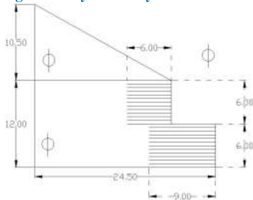
Fig. 5: Drawing of the Reinforced Slope.
