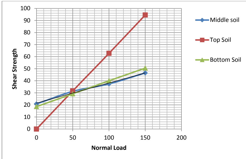
Fig. 3: Graphs from Direct Shear.
